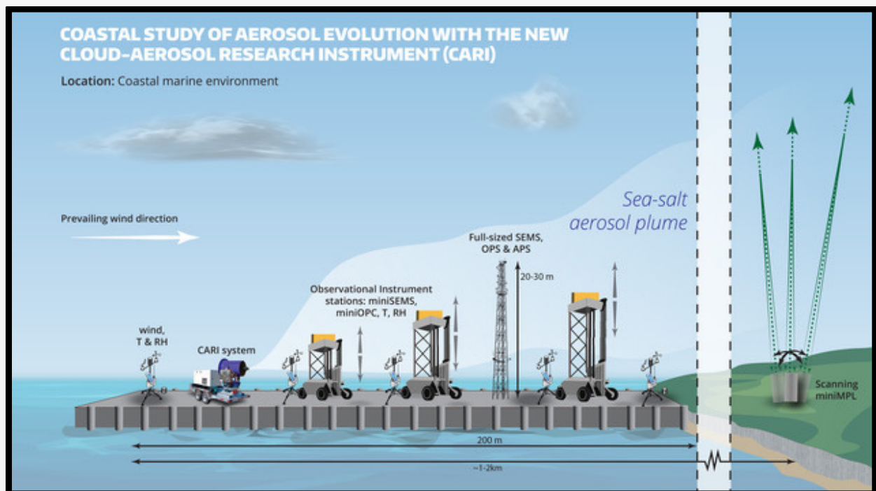
Image 2. Coastal Study of Aerosol Evolution With The New Cloud-Aerosol Research Instrument (CARI). This diagram shows the general layout of instruments for a small-scale sea salt process Study on a pier or similar surface in a coastal zone.
